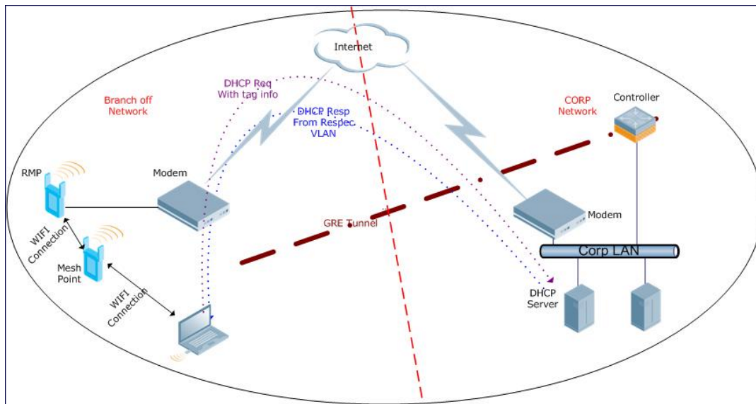
Figure 72 Working of Remote Mesh Portal
