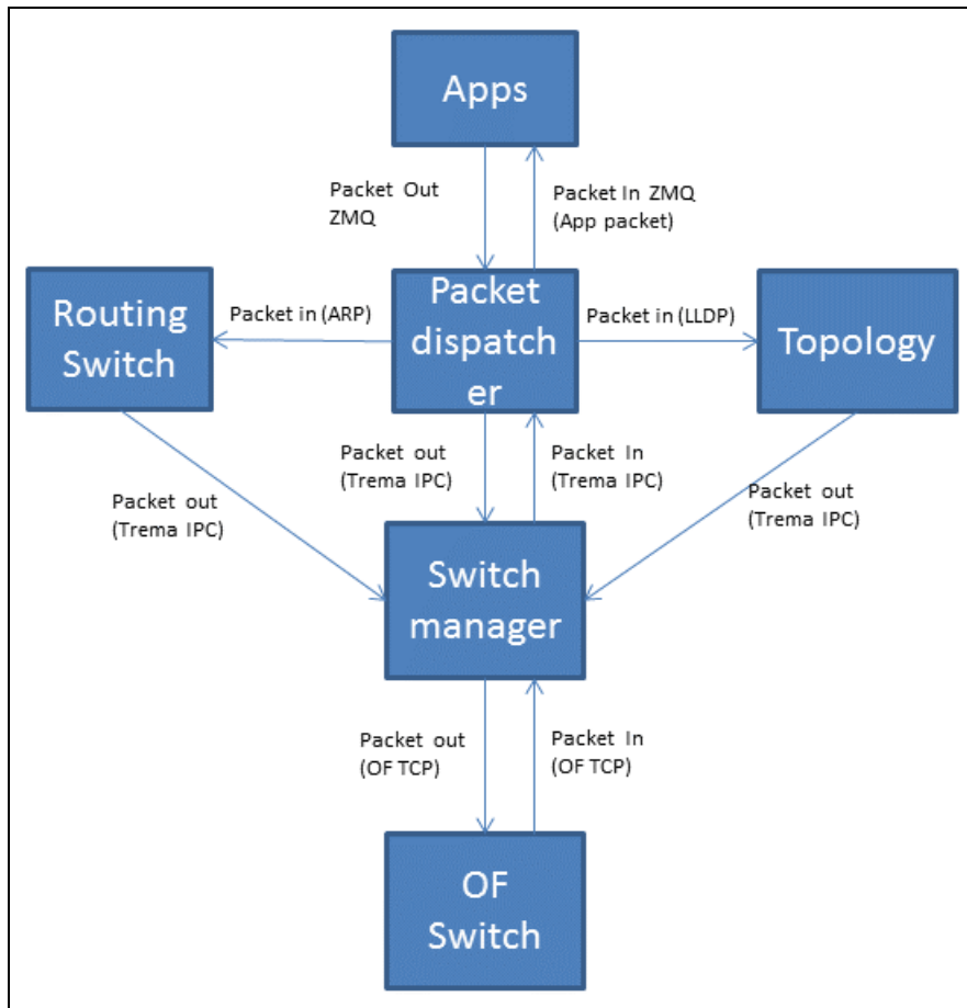
Figure 108 Packet Handling
