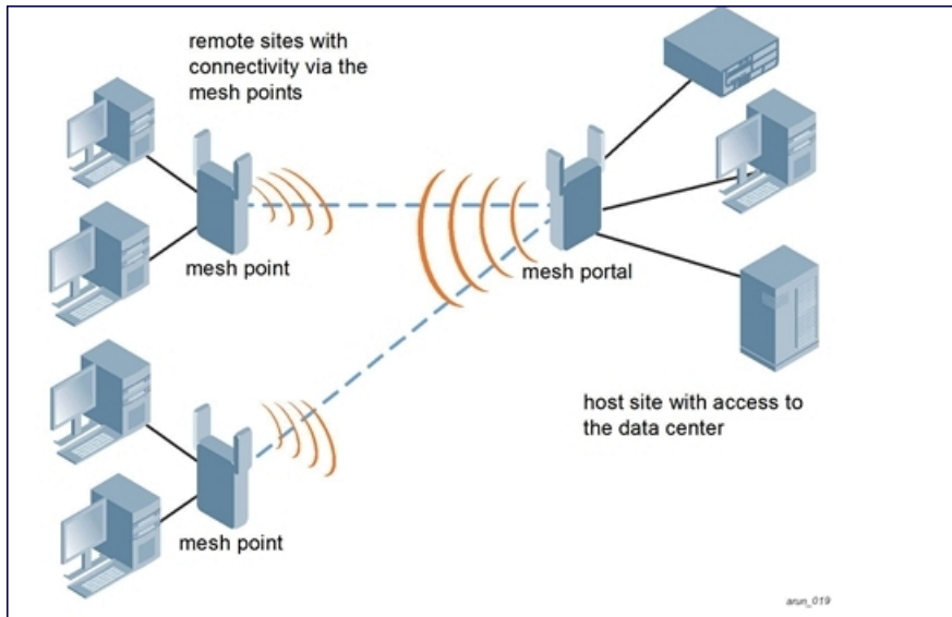
Figure 75 Sample Point-to-Multipoint Deployment
