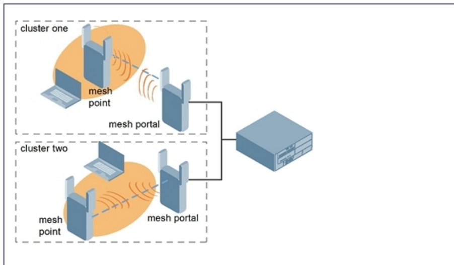
Figure 71 Sample Mesh Clusters
