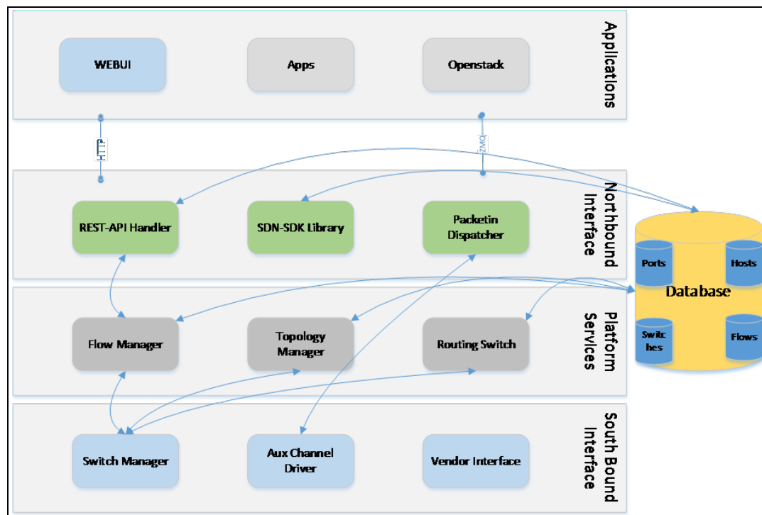
Figure 104 SDN Switch Architecture
