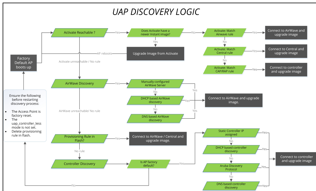
Figure 64 AP Discovery Logic
