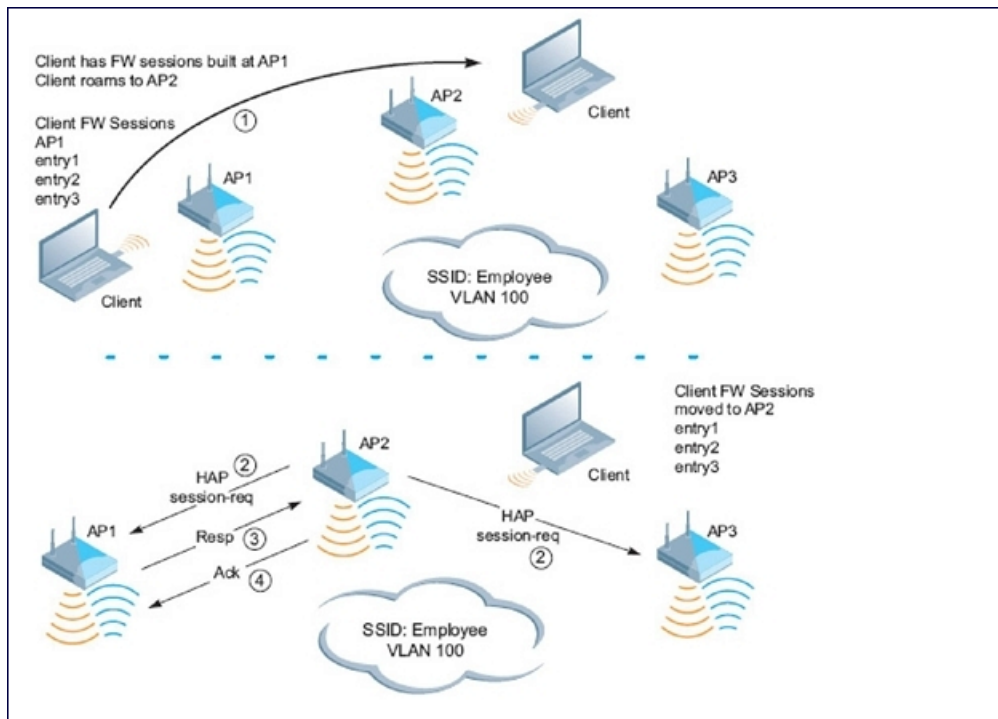
Figure 83 Bridge Mode Mobility
