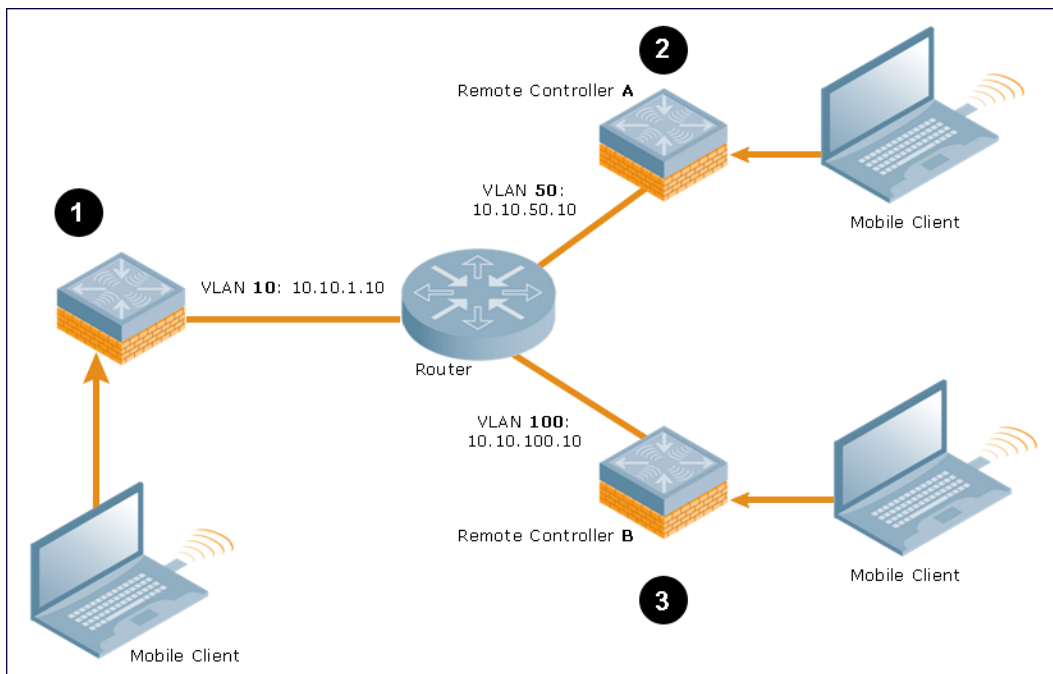
Figure 84 Inter-managed device Mobility
