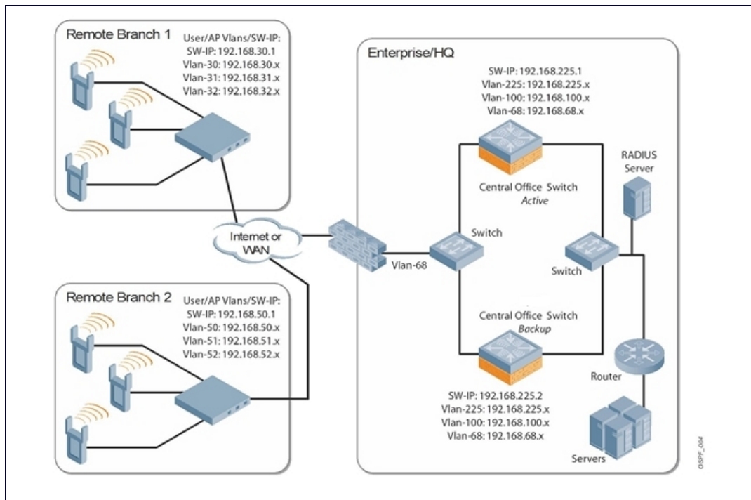
Figure 17 Sample OSPF Topology
