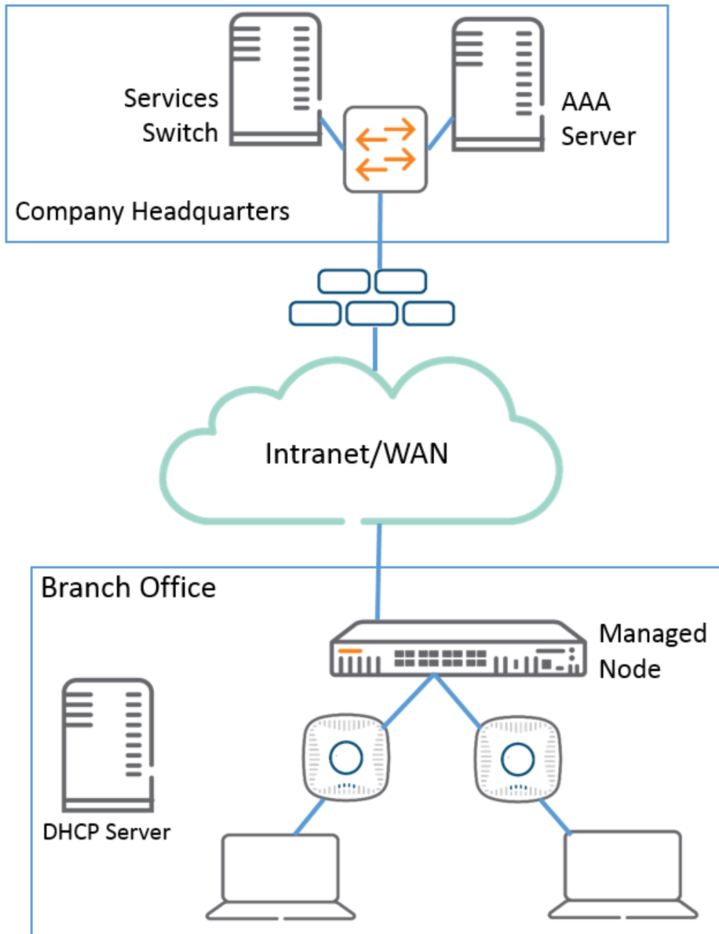
Figure 25 Managed Device Topology
