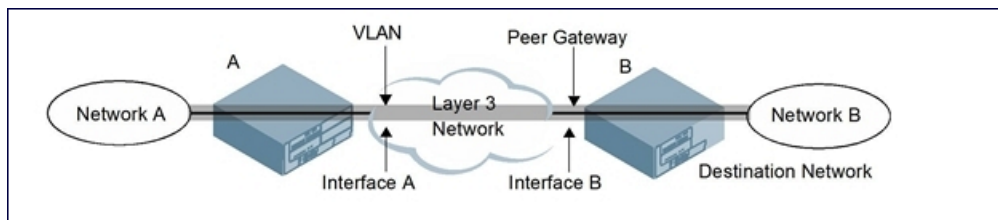
Figure 63 Site-to-Site VPN Configuration Components
