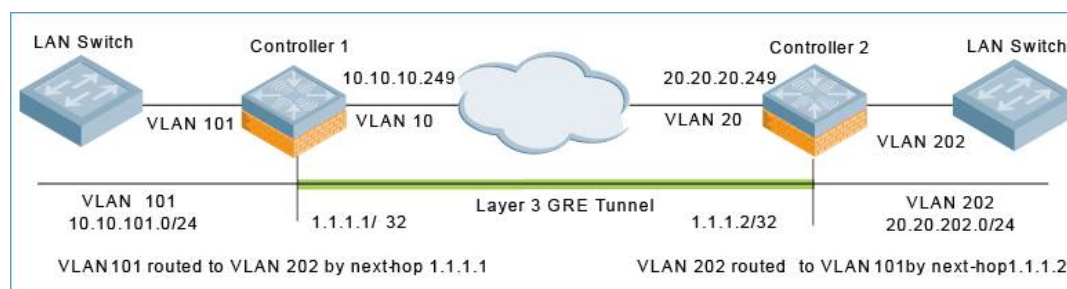
Figure 14 IPv4 Layer-3 GRE Tunnel
