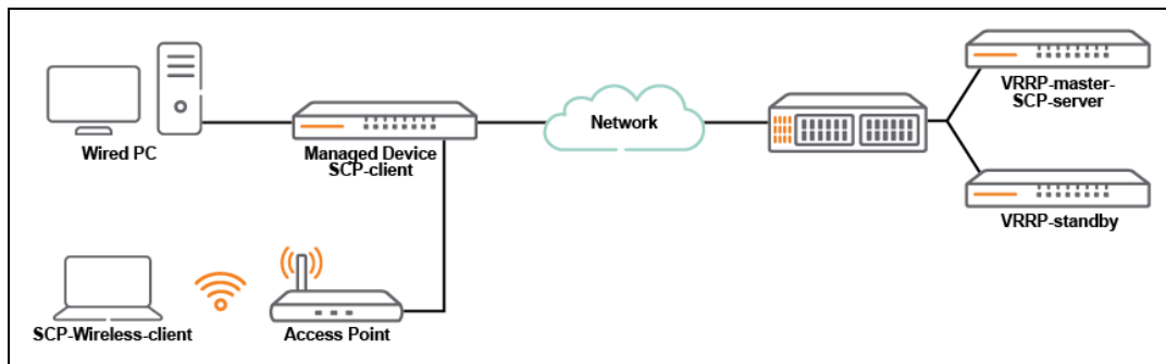
Figure 103 Sample Topology - VRRP Conductor as SCP Server
