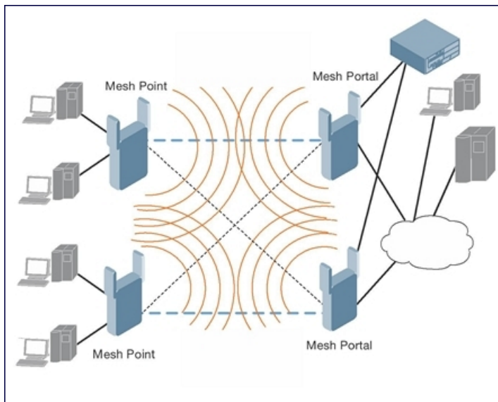
Figure 76 Sample High-Availability Deployment
