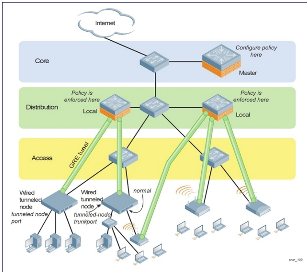
Figure 18 Tunneled Node Configuration Operation
