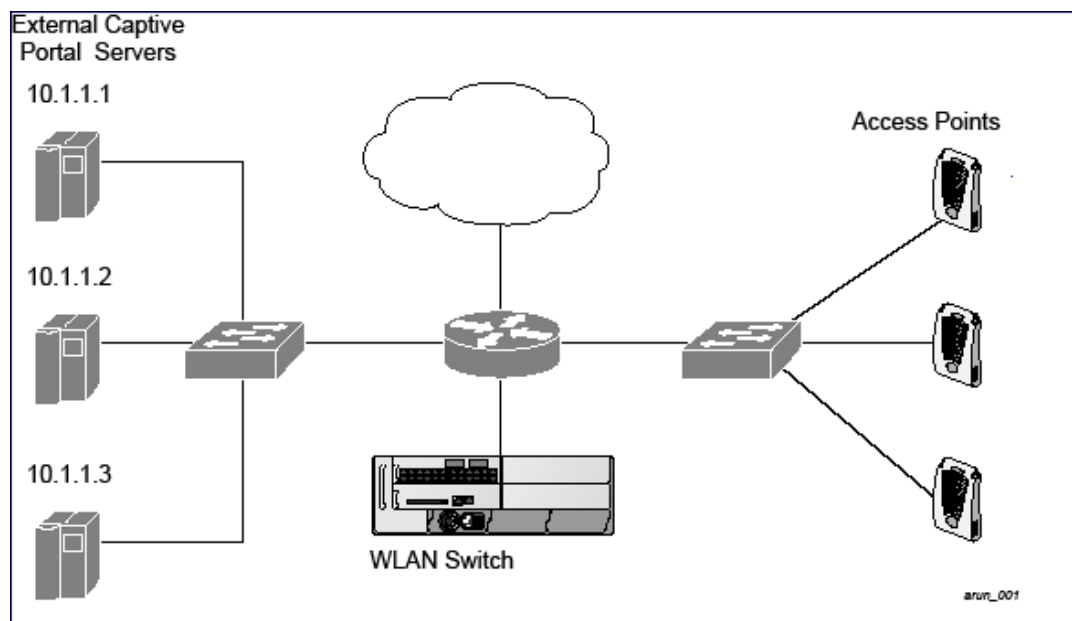
Figure 116 Example NAT-Mode Topology
