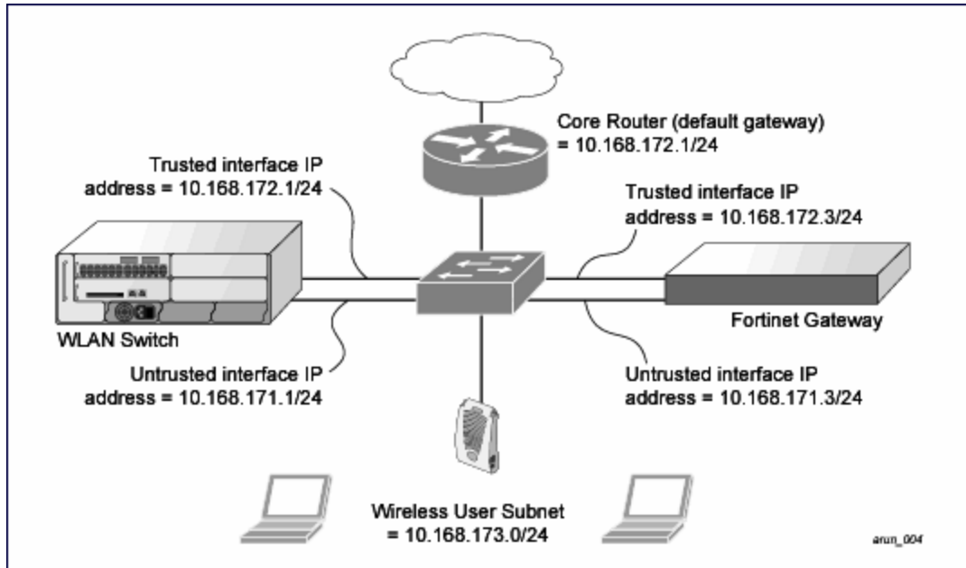
Figure 115 Example Route-Mode Topology
