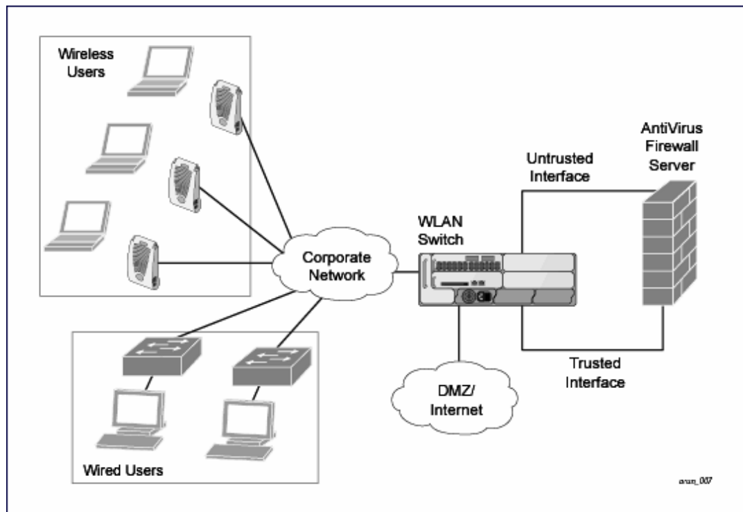
Figure 110 ESI-Fortinet Topology
