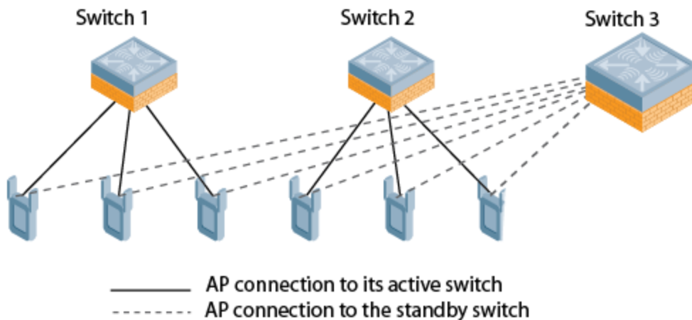
Figure 79 1:1 Active/Standby Deployment
