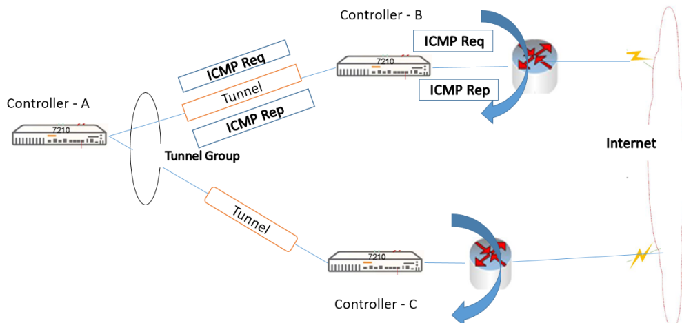
Figure 16 ICMP based GRE Tunnel
