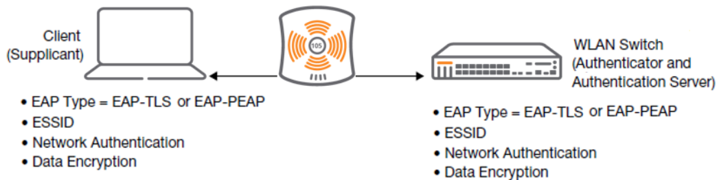
Figure 30 802.1X Authentication with Termination on Managed device
