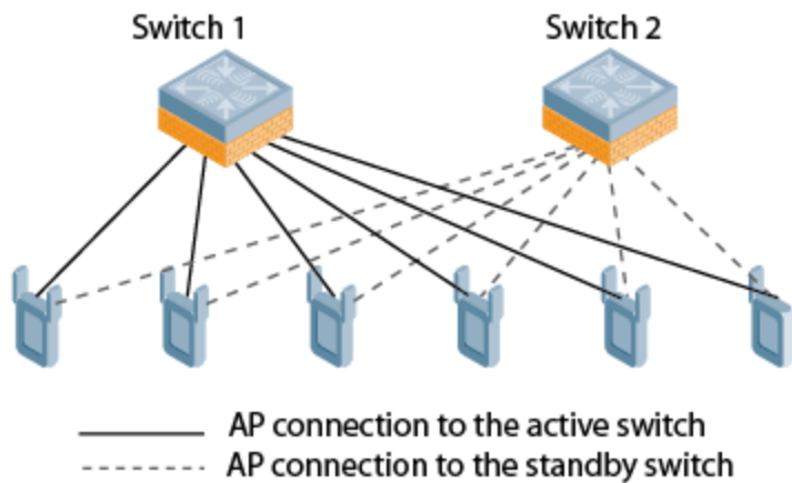
Figure 78 1:1 Active/Standby Deployment
