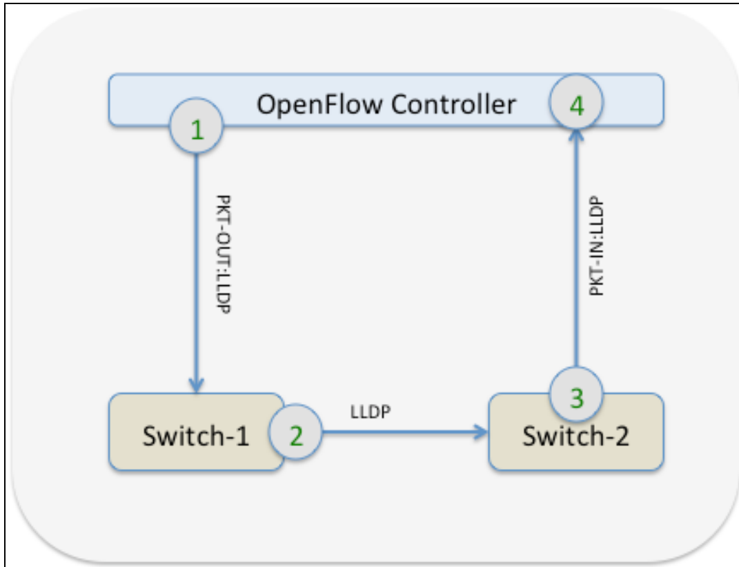
Figure 105 Topology Discovery
