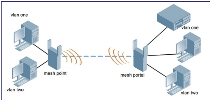
Figure 74 Sample Point-to-Point Deployment
