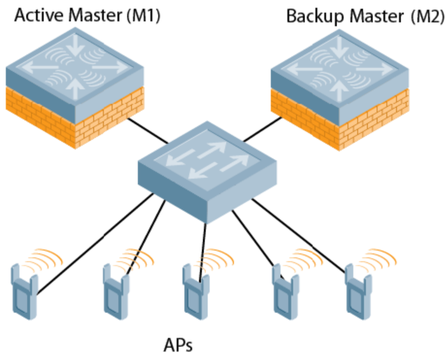
Figure 80 Redundancy with an Active-Backup Conductor Switch Pair
