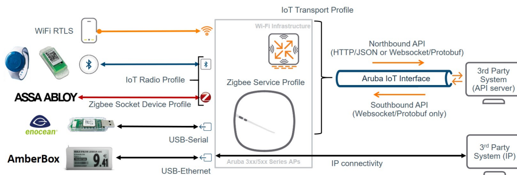
Figure 109 IoT Connectivity
