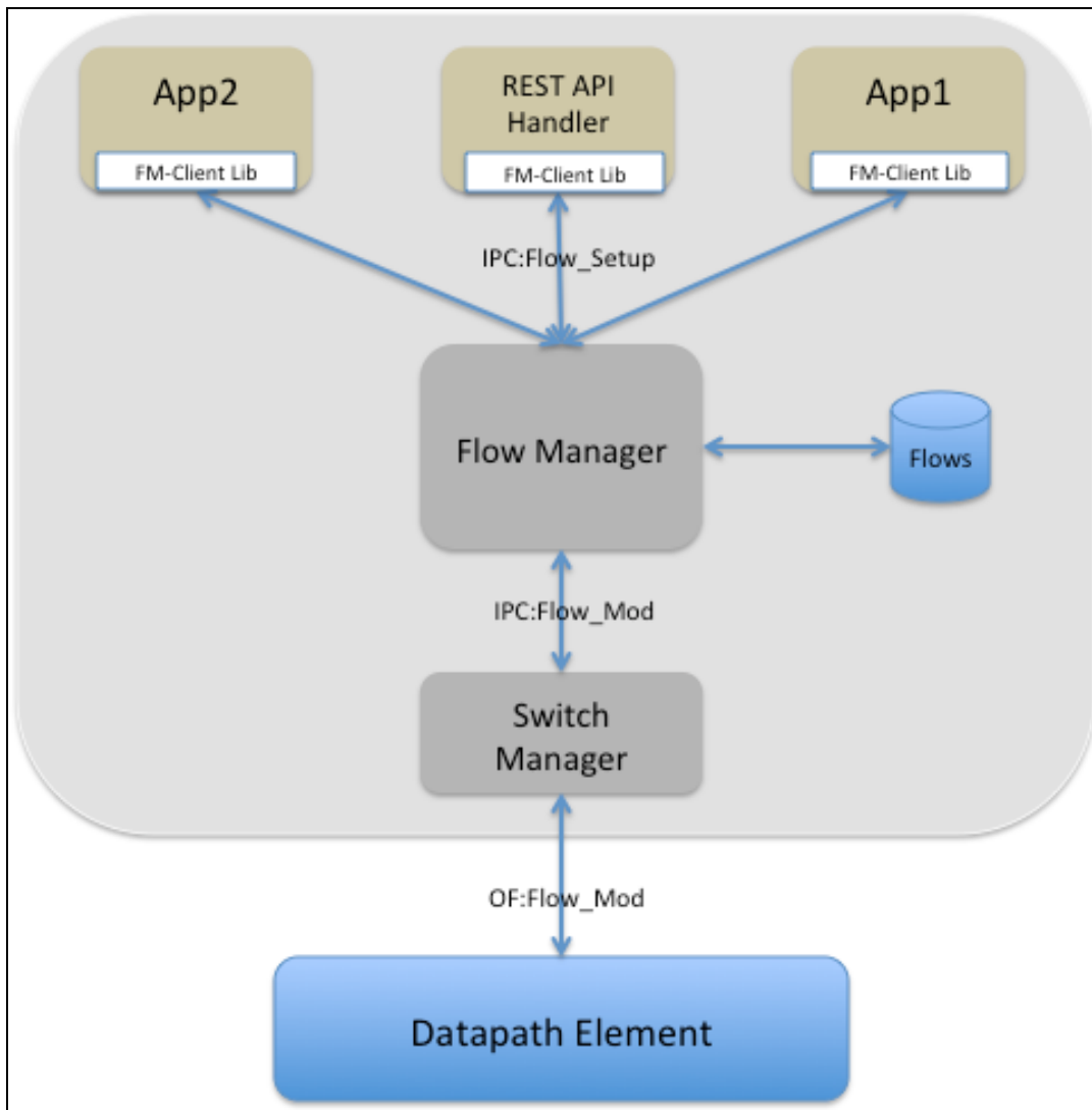
Figure 107 Flow Push
